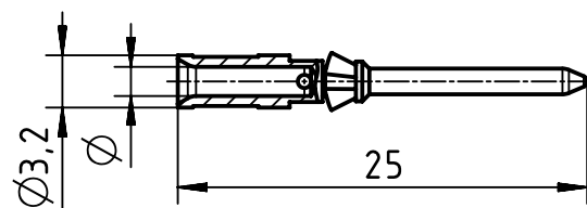
male contact
