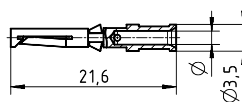
female contact
